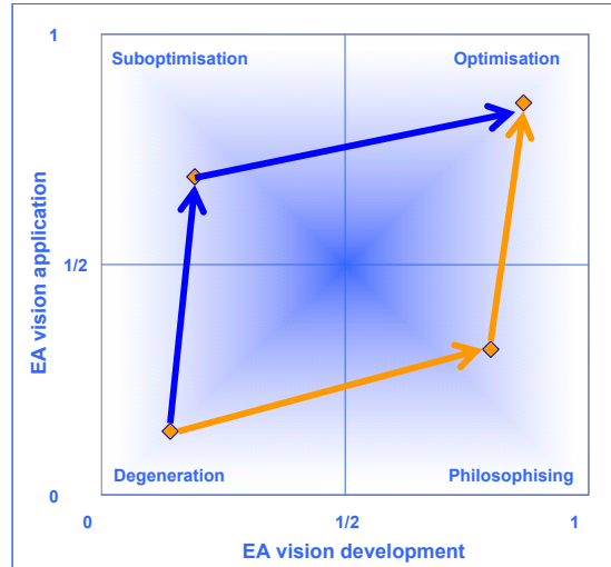
Fig. 7. Development scenarios
